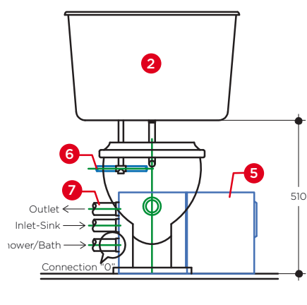
elevation view
