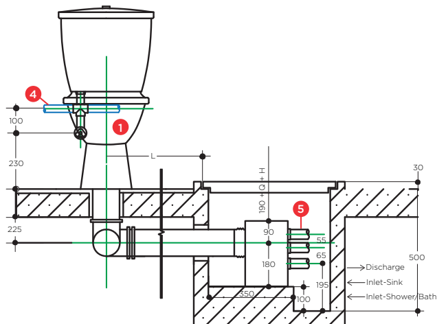
sectional view
